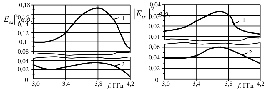
Pic. 1. The square of amplitude of EMF electric component |E_{0z}|^2 versus frequency response f for a pig leg: 1 – in bone marrow area; 2 – in bone tissue area Pic. 2. The square of amplitude of EMF electric component |E_{0z}|^2 versus frequency response f for a cow leg: 1 – in bone marrow area; 2 – in bone tissue area
