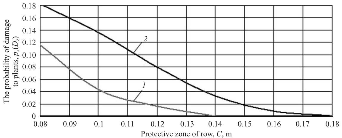
Fig. 6. The probability of damaging the plants \delta_A(D_Z) depending on the scope of the protection zone \tilde{N} : 1 – internal working tool; 2 – external working tool
