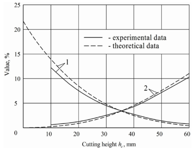
Fig. 4. Dependence of sugar-bearing plant material losses (1) and tops residues (2) on the height cutting without copier h_c
