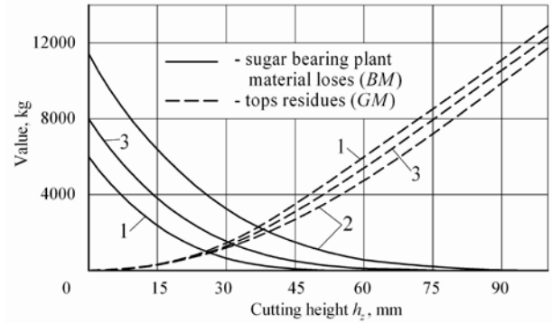
Fig. 3. Dependencies for finding cutting height without copier at expectation value m = 40 mm
