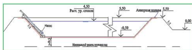
Fig. 6. Profile lagoon project
