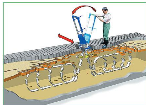
Fig. 3. Mixers for mixing the manure in baths
