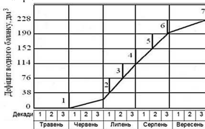
Figure 1 - Integrated supply curve deficit
