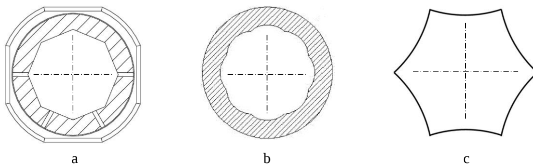
Fig. 24. Cross-section of the single-screw presses barrels press section:
