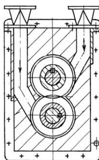
Fig. 10. Cross-section of a twin-screw press with individual screw feeding (Patent Nos. CN1810497A, CN203305535U)
