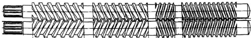
Fig. 8. Scheme of screws of a twin-screw press with multi-directional rotation of screws with cutting sections of the opposite direction (Patent Nos. CN2594005Y, CN205130454U)
