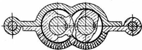
Fig. 20. Cross-section of the working part of a twin-screw press with a assembled barrel (Patent Nos. UA25846C2, RU2108239C1)
