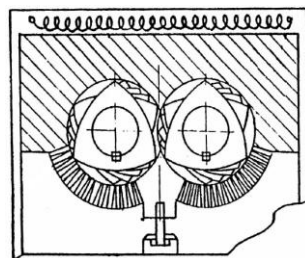
Fig. 21. Cross-section of the working part of a twin-screw press with a assembled barrel (Patent No. UA24490A)
