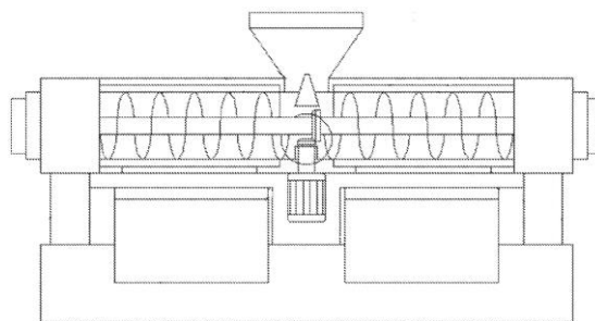
Fig. 4. Single-screw press with two independent press zones (Patent No. CN217916906U)
