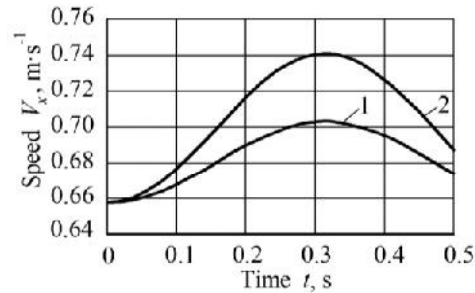
Figure 4. Variation of material particle (seed) velocity V_x as function of t relative to Ox axis: 1 – medium fraction seeds; 2 – heavy fraction seeds.
